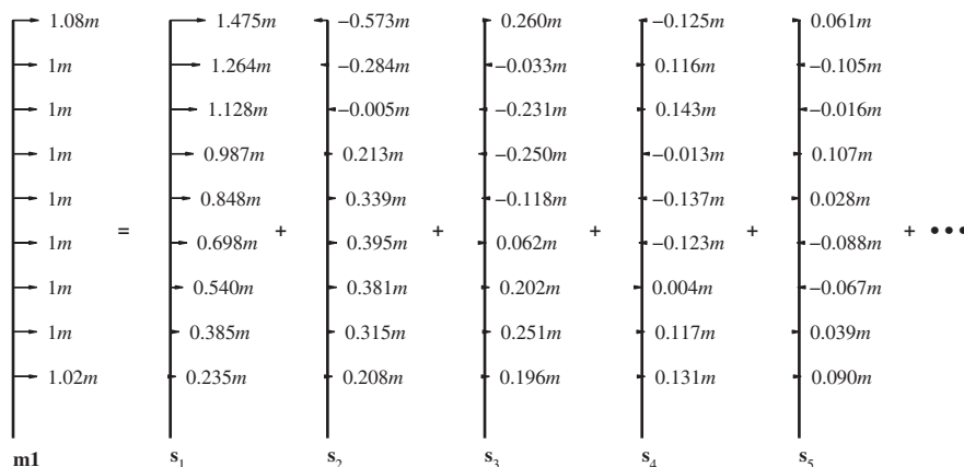
Figure 20.5.2 Modal expansion of the distribution \mathbf{s} = \mathbf{m}\boldsymbol{\mu} of effective earthquake forces.
